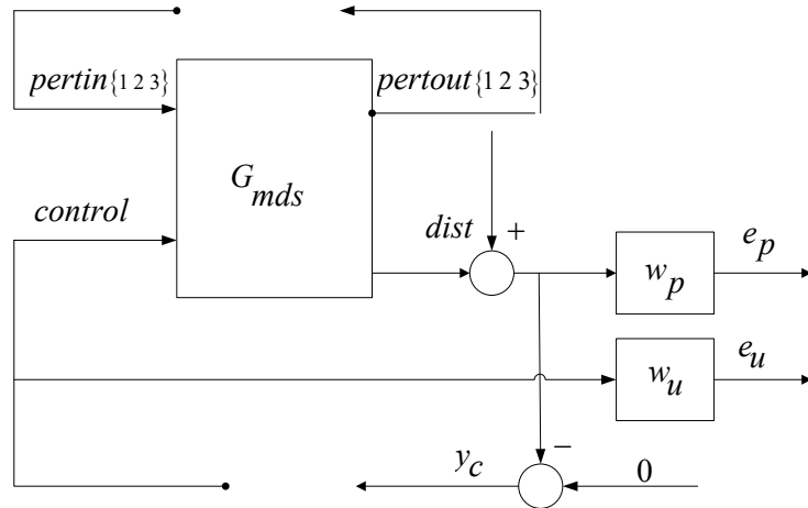
Figure 23: Open loop structure [18]
