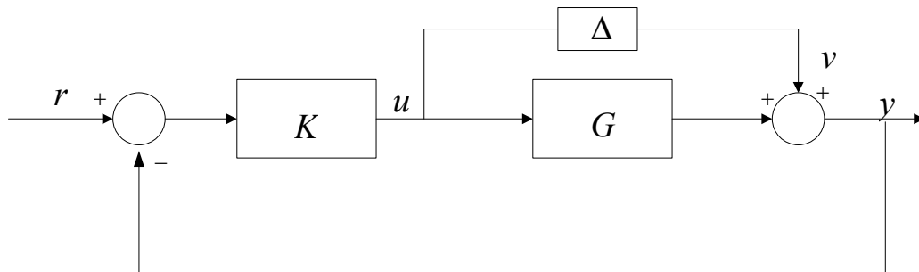
Figure 54: Closed loop feedback system with uncertainty [18]
