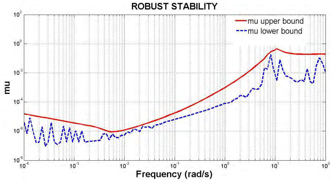
Figure 29: Robust stability for roll rate
