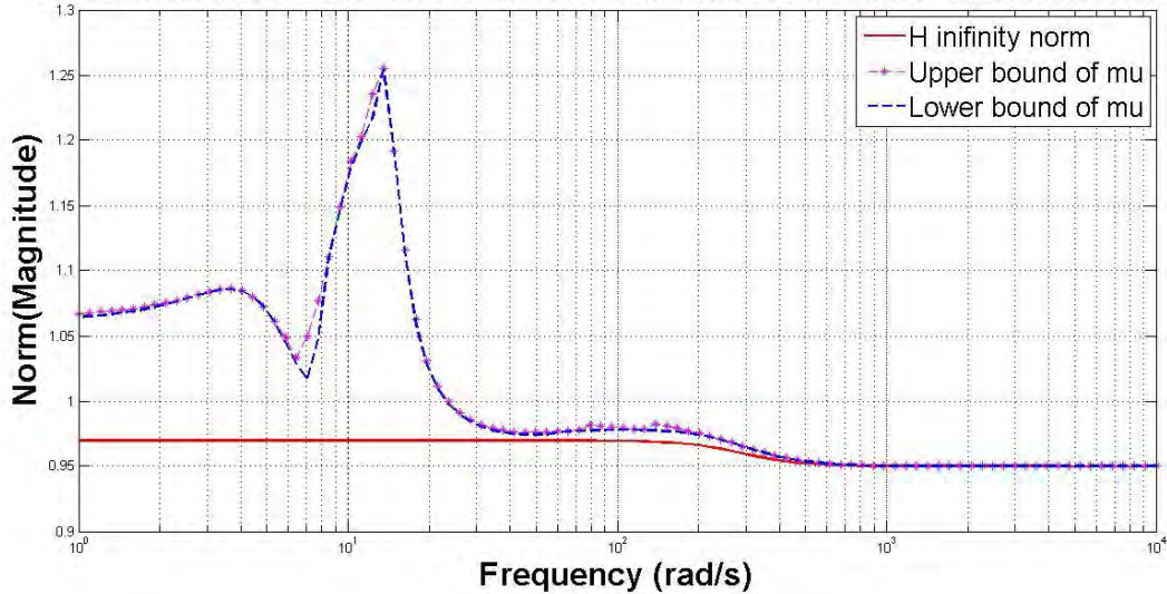
Figure 31: Nominal and robust performance for roll rate
