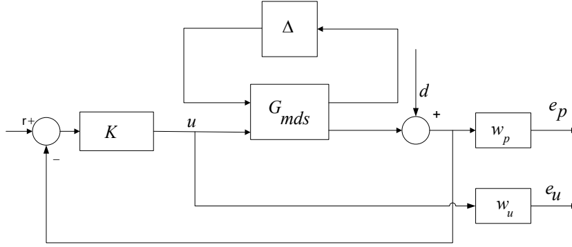
Figure 20: Closed loop system with weighting functions [18, 19]
