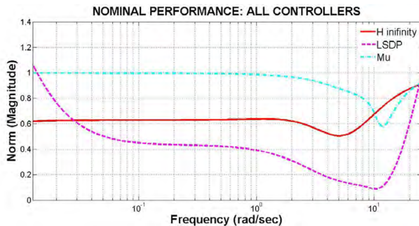
Figure 71: Comparison of nominal performance for all controllers
