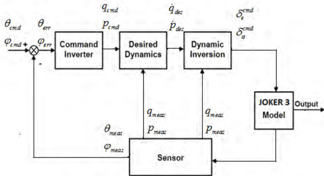
Figure 2: Overall Dynamic Inversion block [15]
