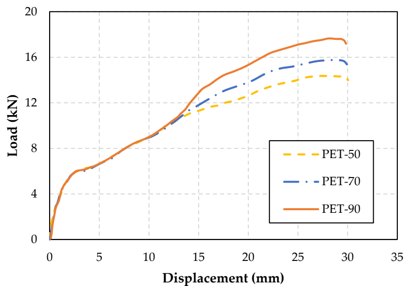
Figure 11. Effect of concrete compressive strength on the behavior of PET-FRP-strengthened slabs.
