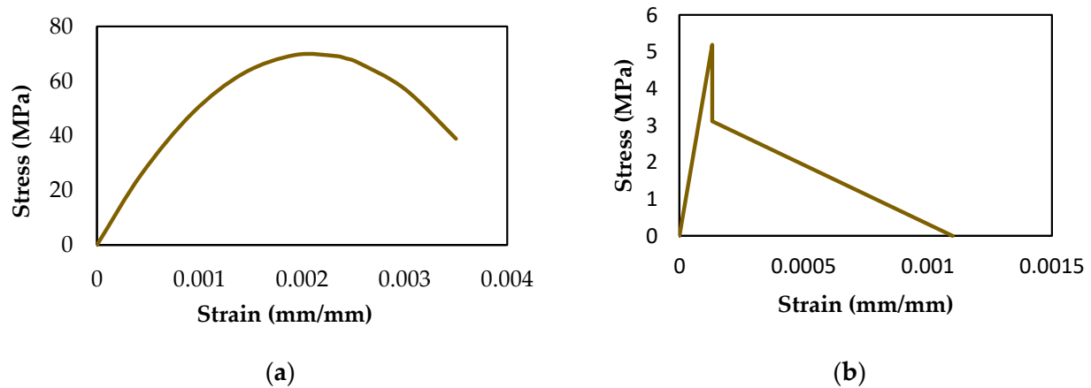
Figure 4. Constitutive models for concrete with f'_c of 70 MPa: (a) Compressive stress-strain curve; (b) tensile stress-strain curve.
