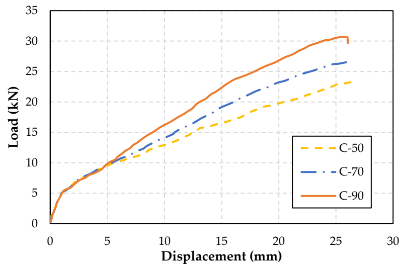
Figure 8. Effect of concrete compressive strength on the behavior of CFRP-strengthened slabs.
