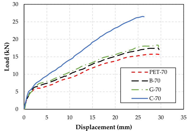
Figure 7. Effect of FRP type on the load-deflection behavior of a strengthened slab specimen.
