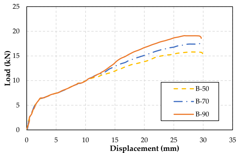
Figure 10. Effect of concrete compressive strength on the behavior of BFRP-strengthened slabs.
