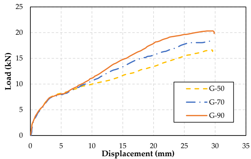
Figure 9. Effect of concrete compressive strength on the behavior of GFRP-strengthened slabs.
