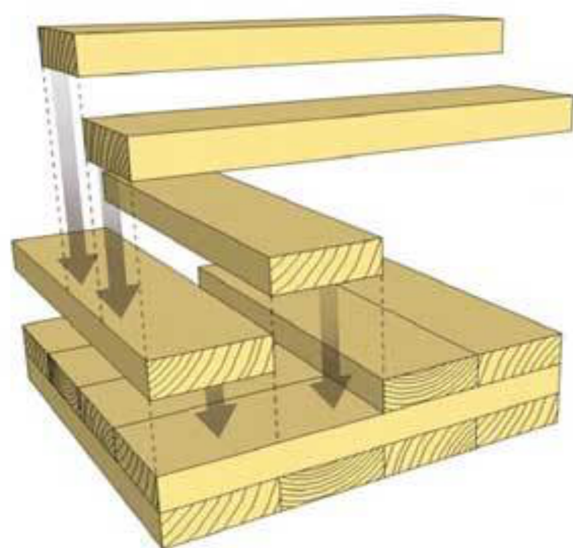
Figure 1: CLT stacking [2]
