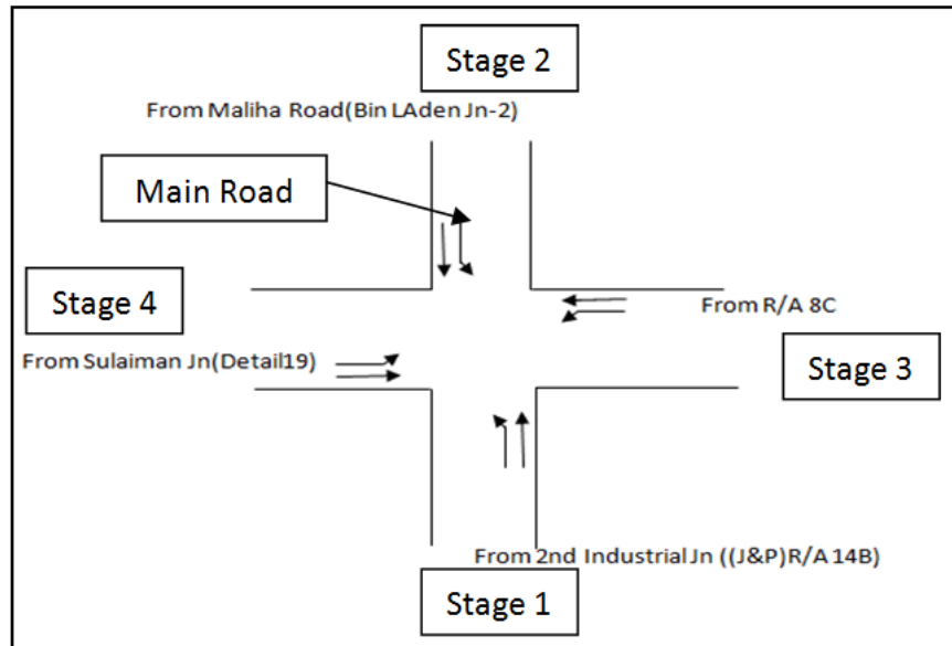
Figure 8: Typical intersection phasing
