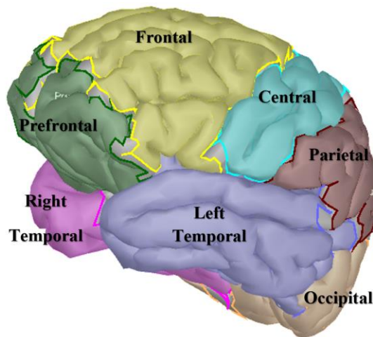
Figure 27: Brain regions for source localization
