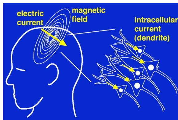
Figure 7: Electromagnetic activity due to intracellular currents [15]
