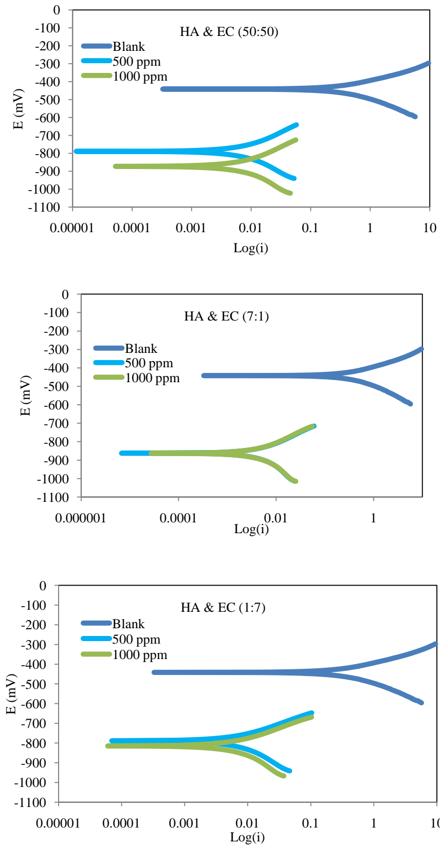
Figure 130: Tafel plots for mild steel in 1 M HCl at 25°C containing different concentrations of mixtures of inhibitors.
