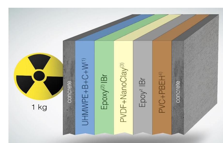
Figure 5: Container Design
