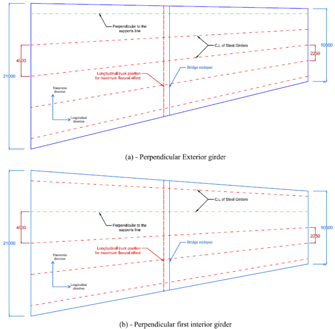
Figure 49: Different splayedness orientations
