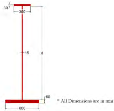
Figure 27: Steel girder dimensions
