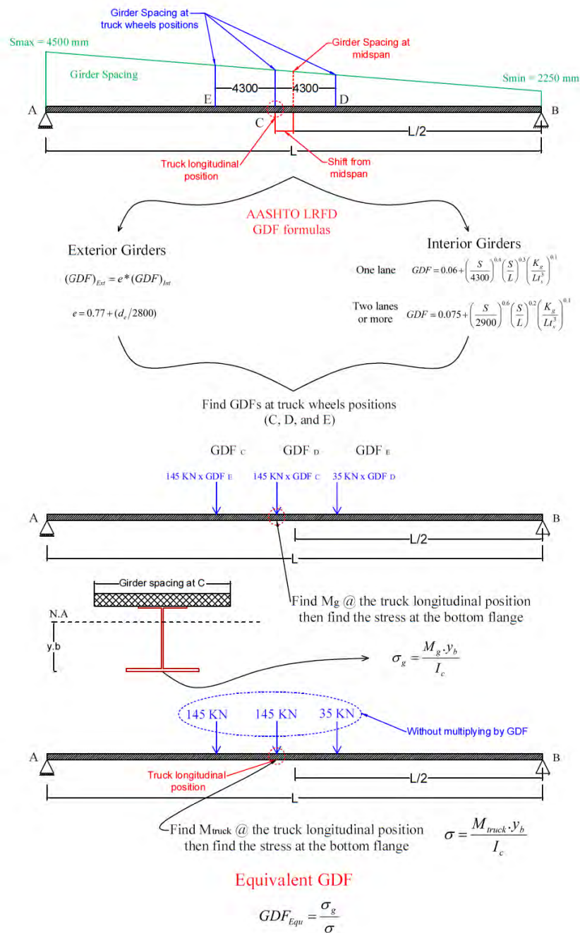
Figure 60: Procedure for calculating the equivalent AASHTO GDF for flexure
