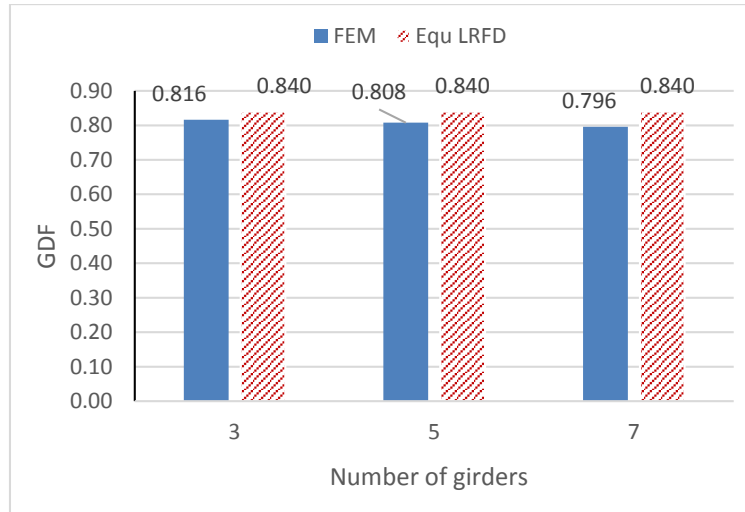
Figure 102: Interior flexure FEM GDF vs. Equ GDF - bridges B1, B10, B11
