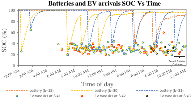
Fig. 13. (a) The SOC and the type of EVs arrivals, and (b) the SOC of a sample of three batteries in the rolling horizon scheduling case of BSS.
