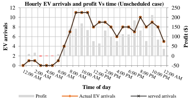
Fig. 8. The profit and the number of EV arrivals at each hour in the unscheduled operation case study.
