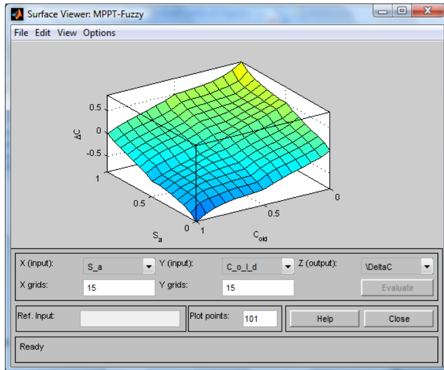
Figure 5.18: Surface viewer MATLAB window
