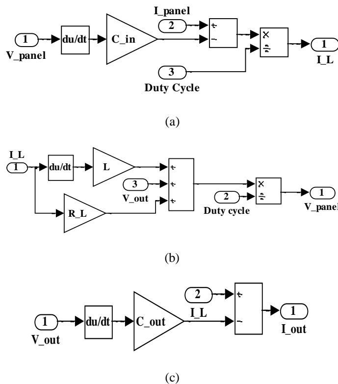
Figure 5.7: a) Buck converter inductor current representation b) Buck converter input voltage representation c) Buck converter output current representation
