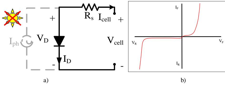
Figure 3.2: a) The un-illuminated junction circuit b) The un-illuminated junction characteristic
