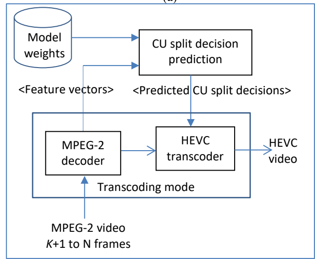
Figure 2. MPEG-2 to HEVC transcoding architecture (a) Training phase (b) Transcoding phase
