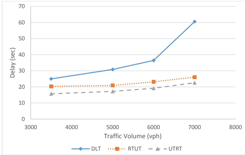
Figure 31: Comparison of Delay for Case 200.I.2
