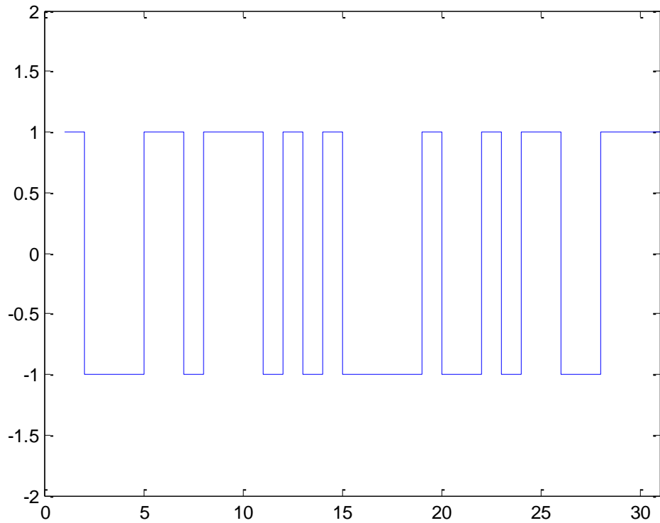
Figure 5.1: Pseudo-random noise derived from an m-sequence.
