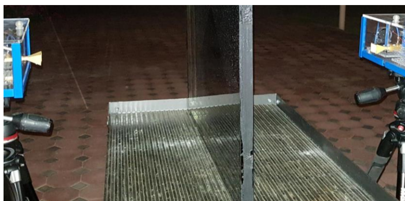
Figure 4.2: Image of one of the penetration loss measurement set up.
