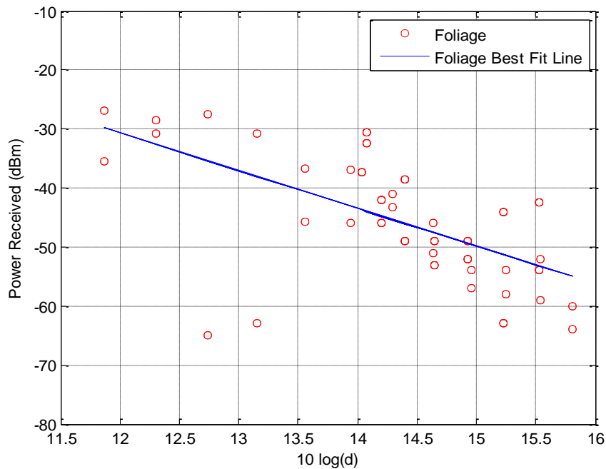
Figure 3.31: Received power measurements in Foliage Environment where TX height is 7.5 meter.
